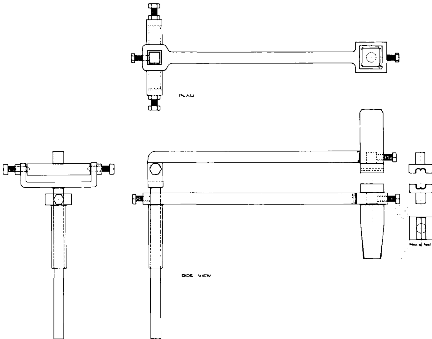
Hinged appliance for top and bottom tools
