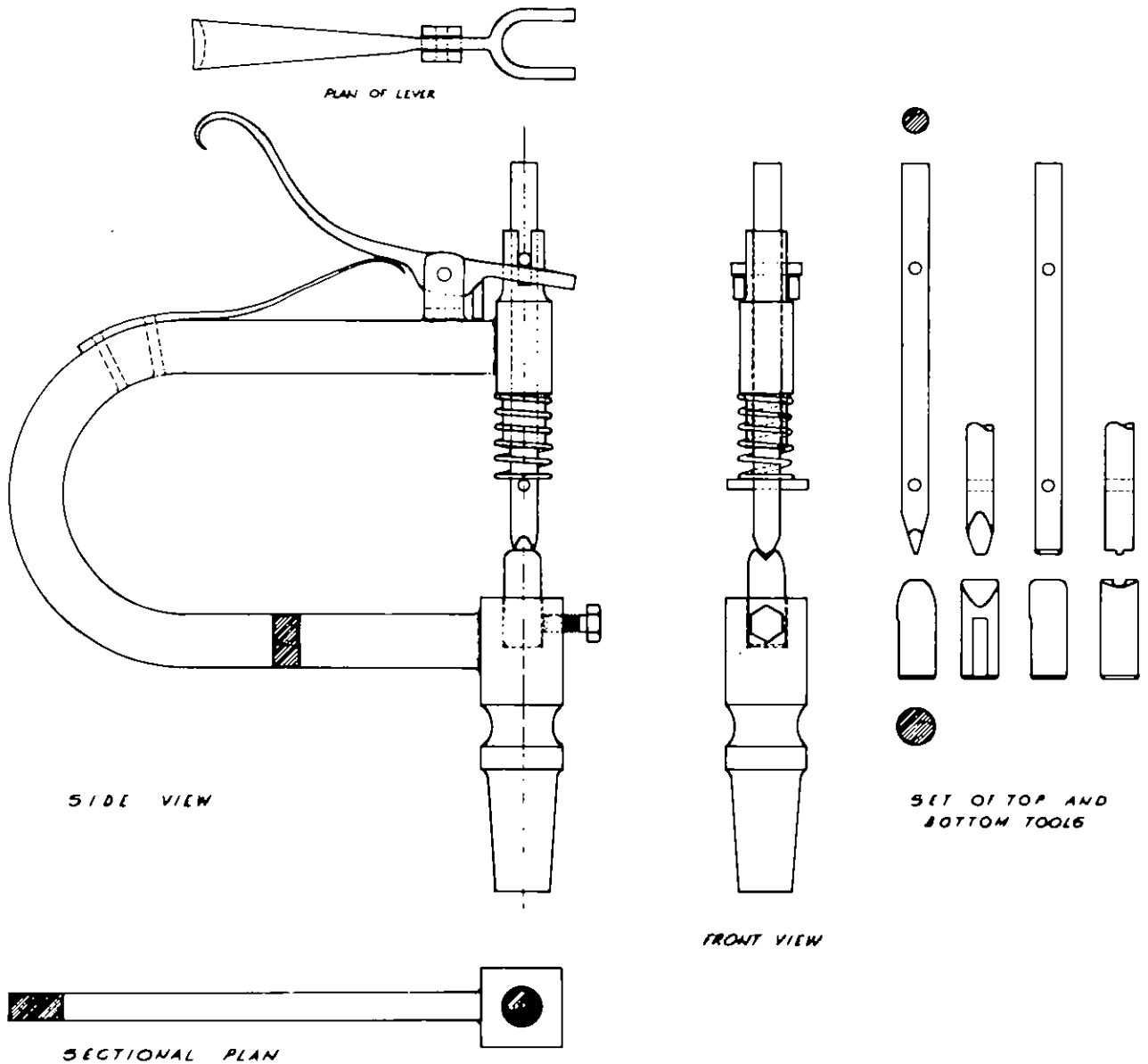
Spring tool for leaf veining
