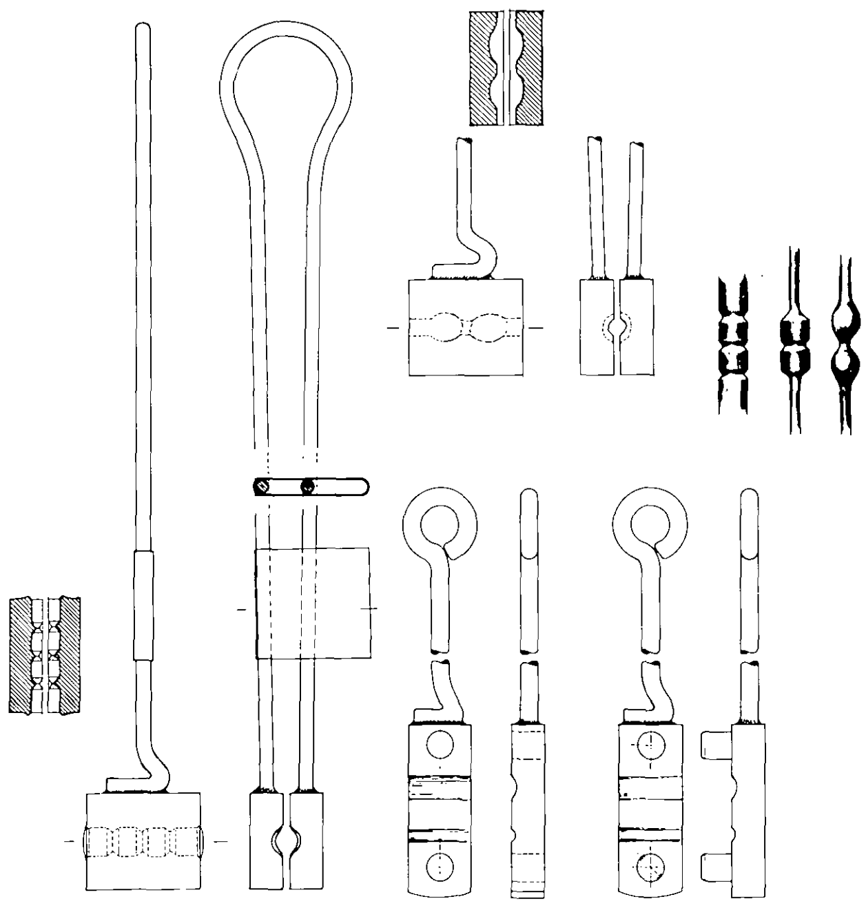
Set of three power hammer tools
