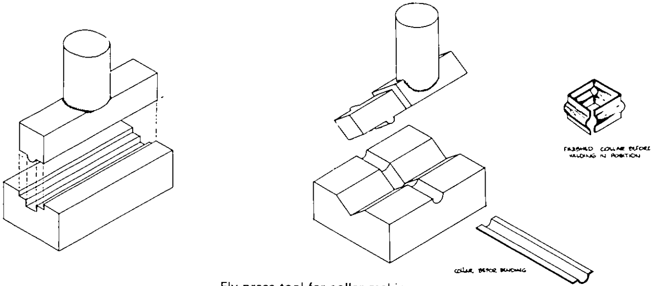
Fly press tool for collar making
